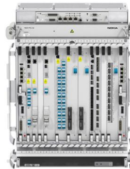
Nokia 1830 PSS-32
